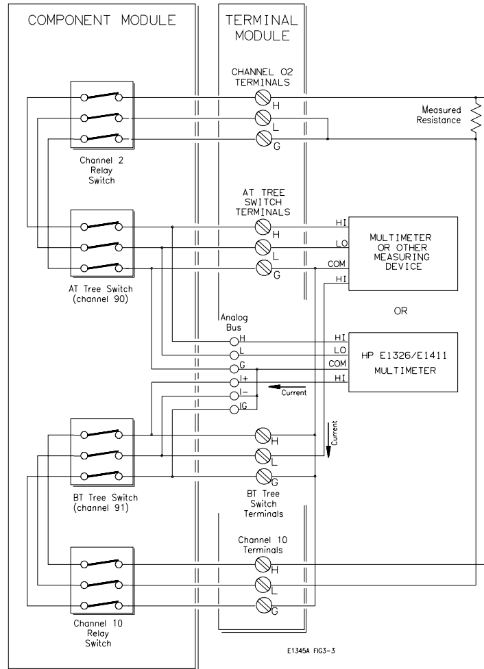
Figure 3-3. Closing Channels 02 and 10 for a 4-Wire Ohms Measurement
